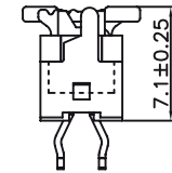
Mating Height Draw.
