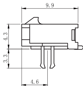
Metallic Peg
